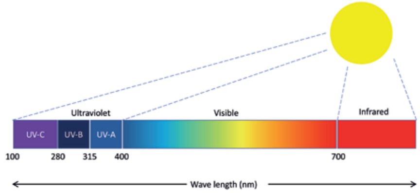
Sunlight spectrum
