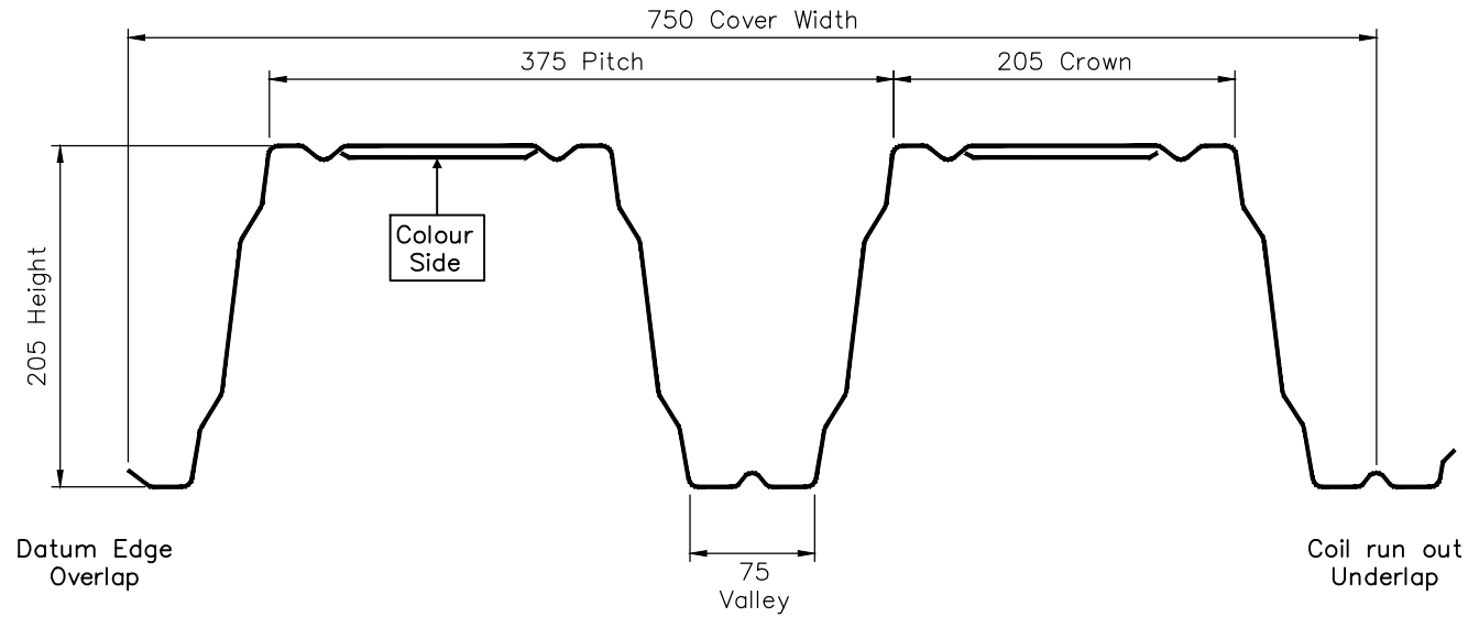
SECTION THROUGH PROFILE
