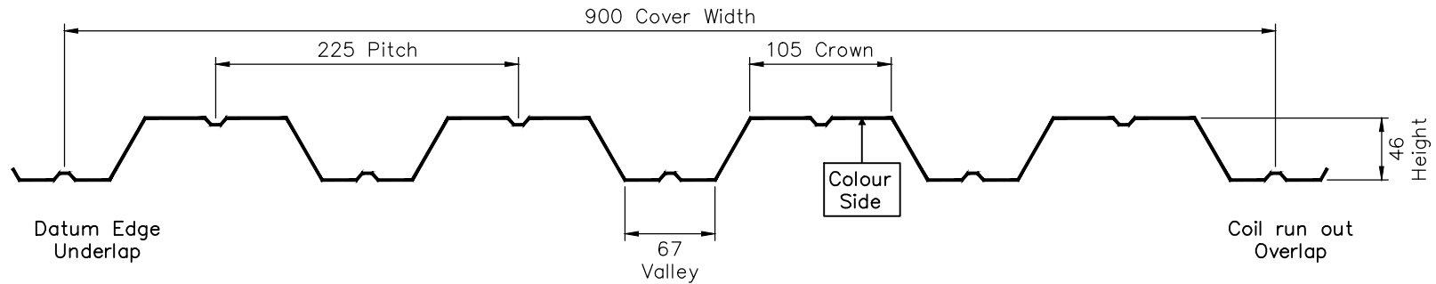
SECTION THROUGH PROFILE
