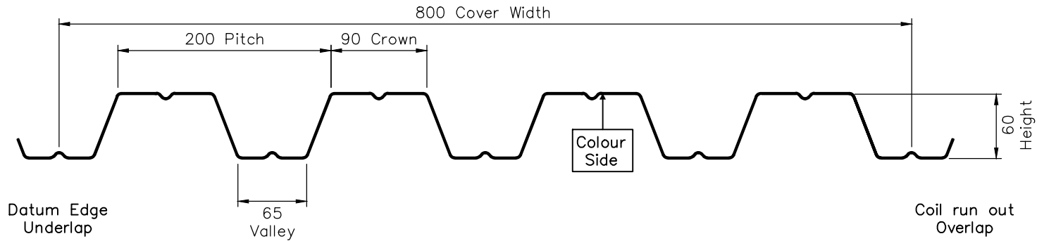
SECTION THROUGH PROFILE
