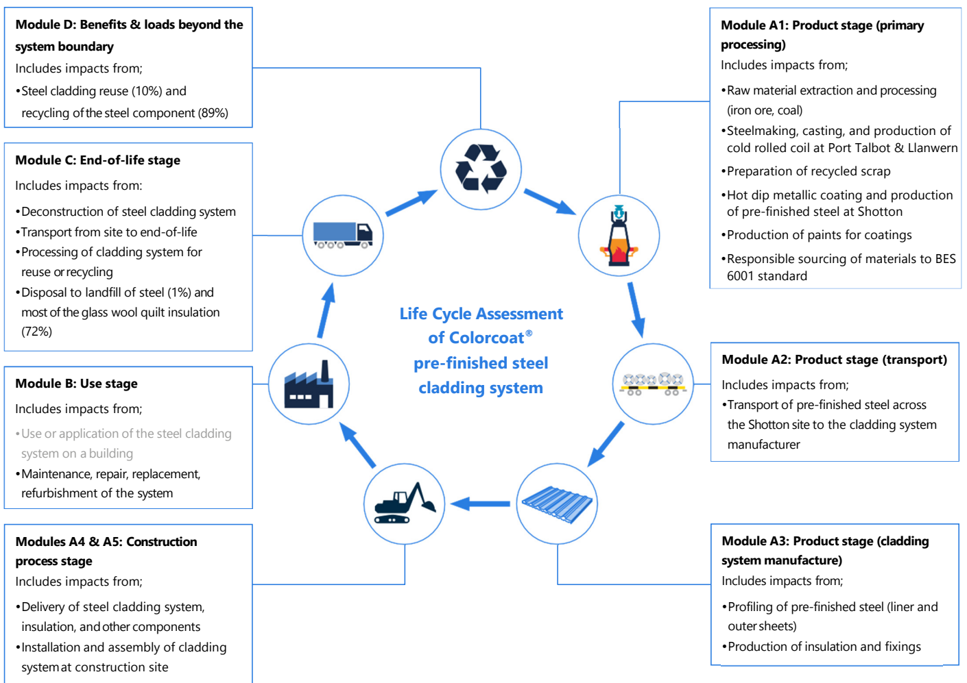
Figure 3 Life Cycle Assessment of steel cladding system
